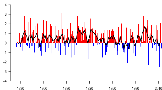
Figure 39 North Atlantic Oscillation (NAO) index
